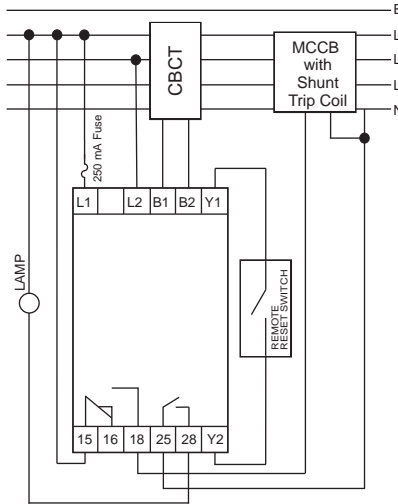
NON-FAIL SAFE MODE WITH SHUNT TRIP COIL
