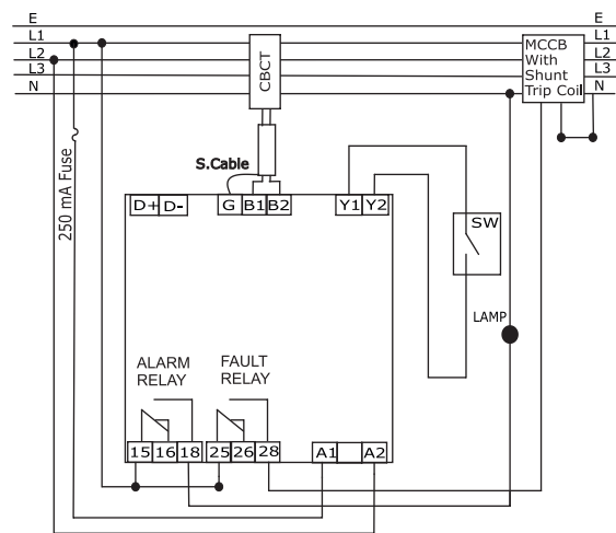
THREE PHASE APPLICATION
