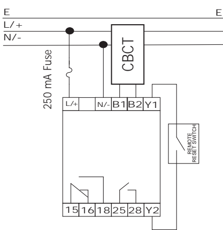
SINGLE PHASE APPLICATION
