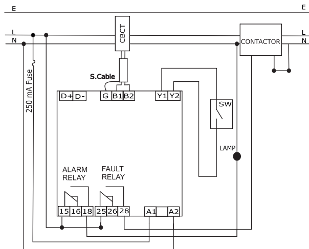
SINGLE PHASE APPLICATION
