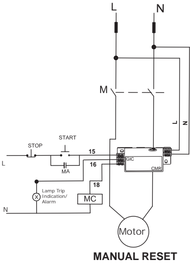
CONNECTION DIAGRAM
