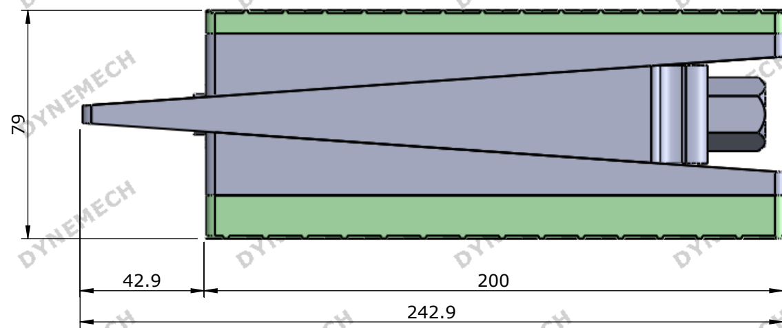
WEDGE MOUNT DF4-u MAX. HEIGHT
