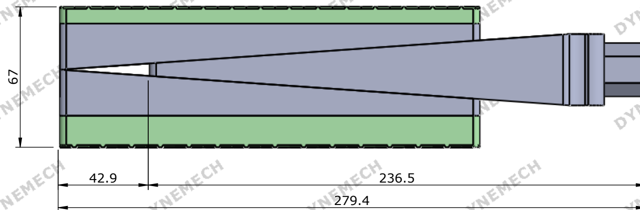
WEDGE MOUNT DF4-u MIN. HEIGHT
