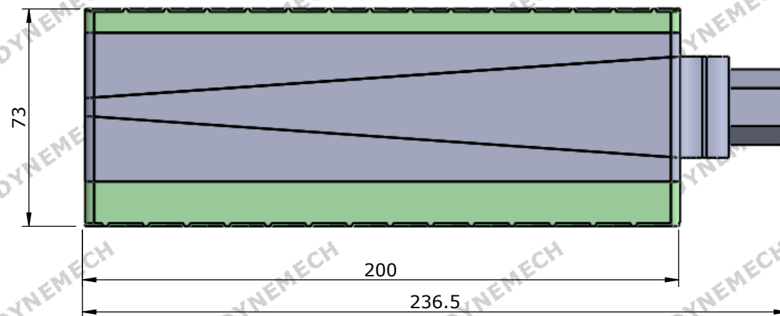
WEDGE MOUNT DF4-u INITIAL HEIGHT
