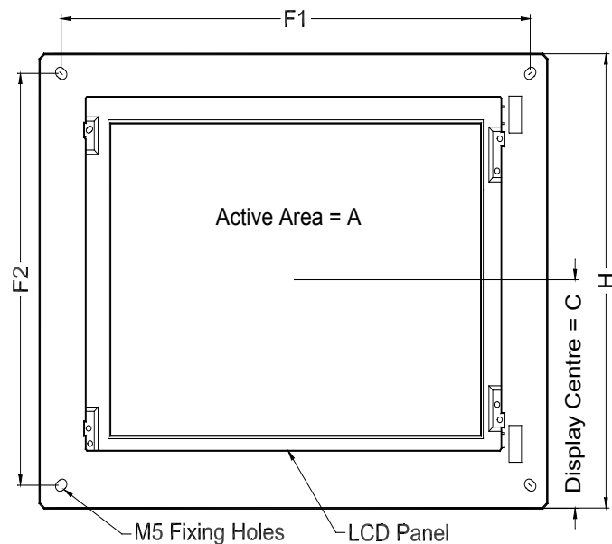
REAR VIEW
