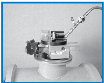
Cutting O-ring and seal groove
