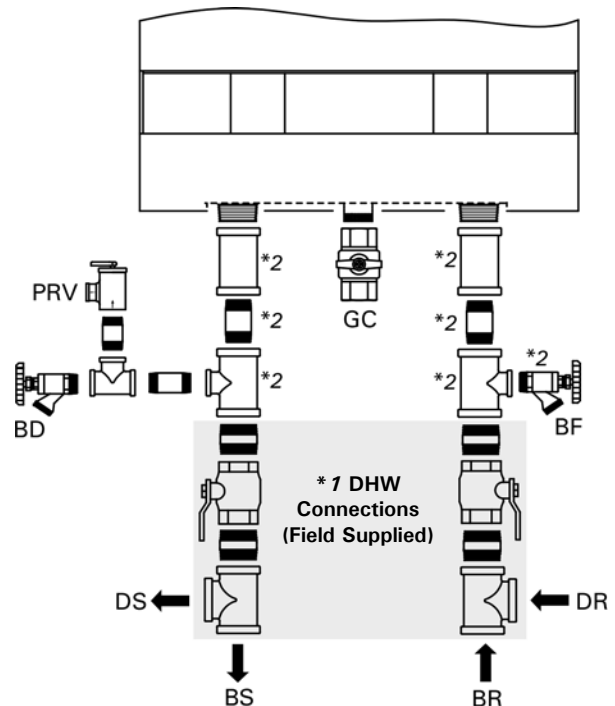
Connections for models B2HA 112 and 150
