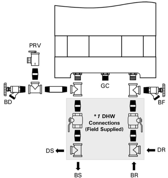
Connections for model B2HA 88 and 100
